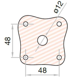
Frontal fixing with 4 screws
