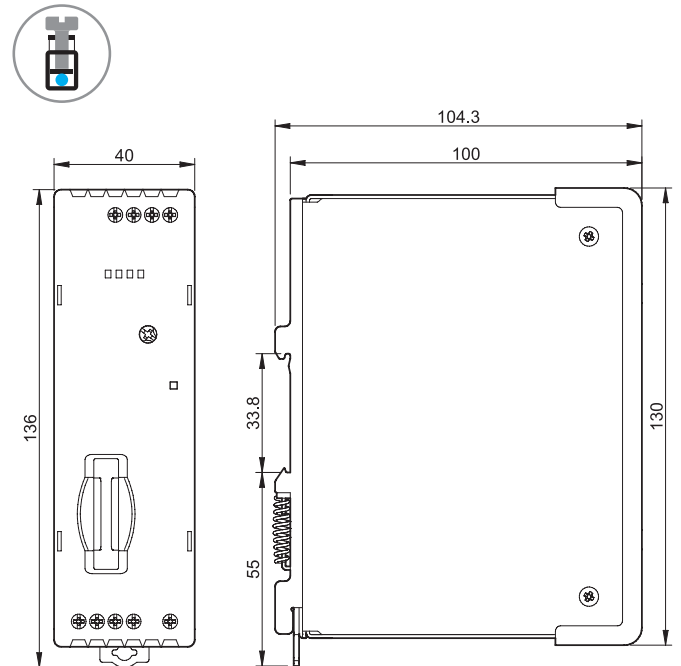
Type 78.1B Screw terminal
