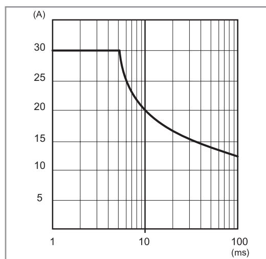
P782E-1 Output peak current v time (78.2E)
