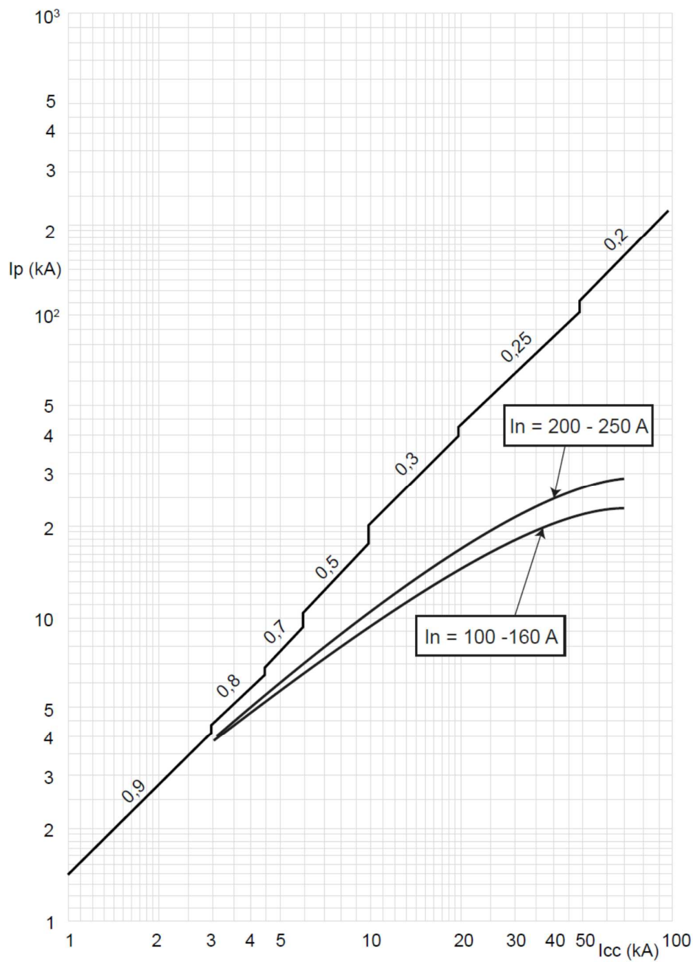
8.3 Cut-off peak current characteristic curve (kA)
