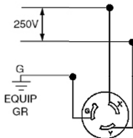
Wiring Diagram
