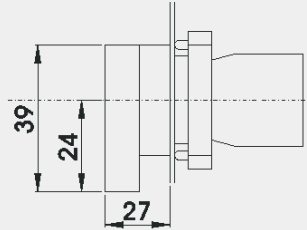
RB2-BJ2+RB2-BZ10 \diamond =RCB2-BJ2 \diamond RB2-BJ3+RB2-BZ10 \diamond =RCB2-BJ3 \diamond
