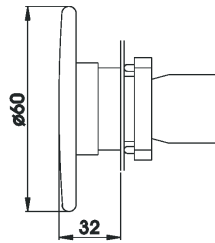
RB2-BS64+RB2-BZ10 \diamond =RCB2-BS64 \diamond
