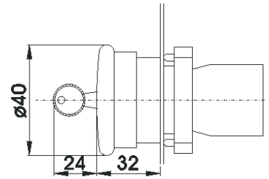
RB2-BS14+RB2-BZ10 \diamond =RCB2-BS14 \diamond
