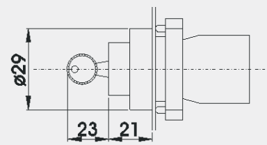
RB2-BG \blacklozenge +RB2-BZ10 \diamond =RCB2-BG \blacklozenge \diamond Replace \blacklozenge with code for position of Key removal & operation pattern
