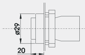
RB2-BL \bullet +RB2-BZ10 \diamond =RCB2-BL \bullet \diamond
