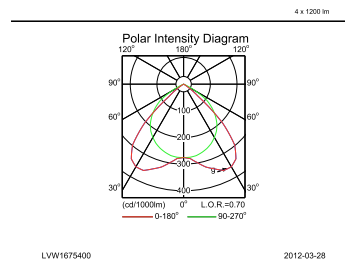
TBS165 G 4xTL5-14W HFS C6
