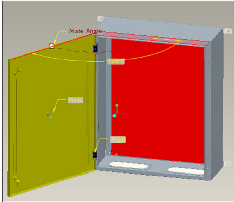
Box with Concealed Hinge and door opening 120 Degree.
